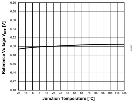
Figure 33 Reference Voltage V_{REF}
