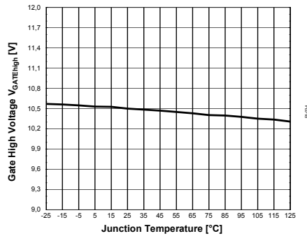
Figure 54 GATE High Voltage V_{GATEhigh}
