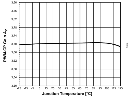
Figure 36 PWM-OP Gain A_V
