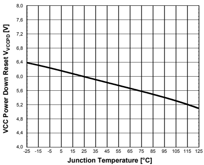
Figure 47 Threshold Power Down Reset V_{VCCPD}
