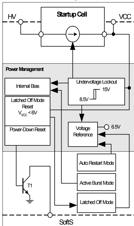
Figure 4 Power Management
