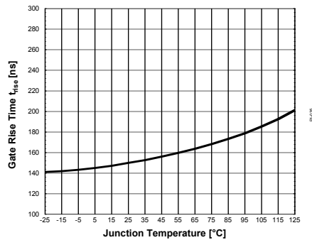
Figure 55 GATE Rise Time t_{rise}
