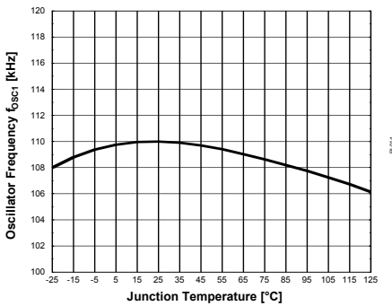
Figure 34 Oscillator Frequency f_{OSC1}
