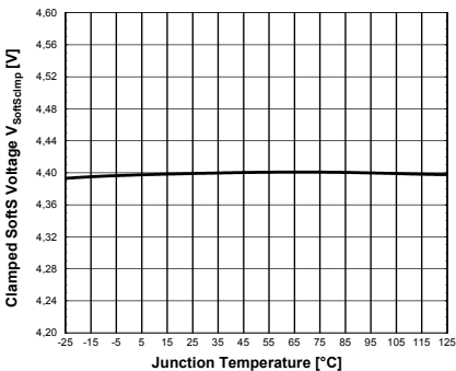
Figure 41 Clamped SoftS Voltage V_{SoftSClmp}
