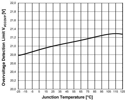
Figure 46 Overvoltage Detection Limit V_{VCCOVF}
