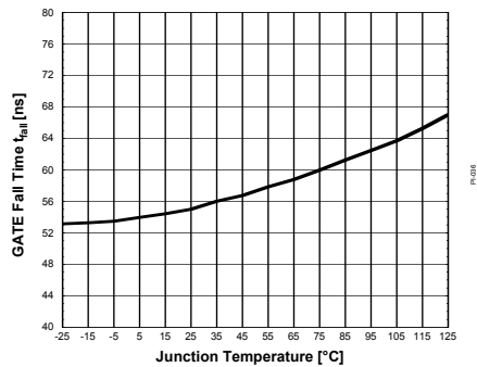
Figure 56 GATE Fall Time t_{fall}
