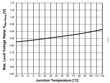
Figure 37 Max. Level Voltage Ramp V_{Max-Ramp}
