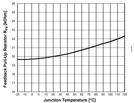
Figure 38 Feedback Pull-Up Resistor R_{FB}
