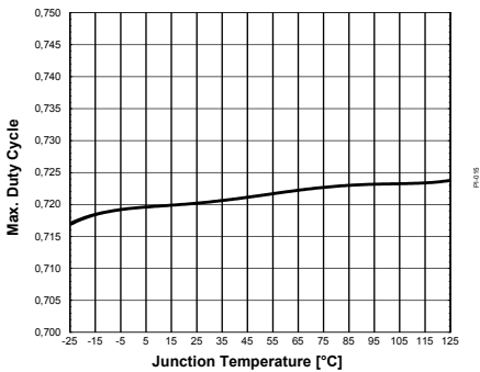
Figure 35 Max. Duty Cycle D_{max}
