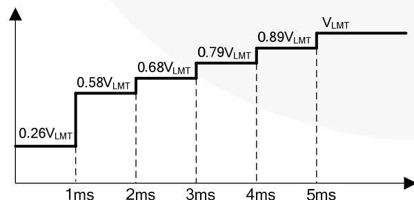
Figure 27. Soft-Start Function
