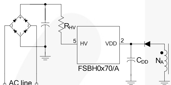
Figure 26. Startup Circuit
