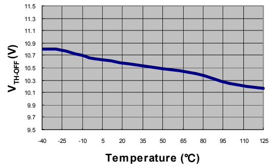
Min. Operating Voltage vs Temperature
