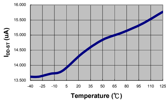
Start-up Current vs Temperature
