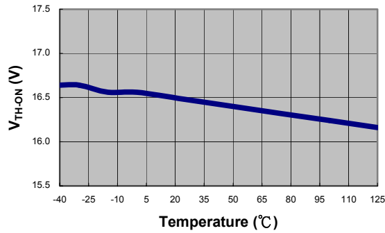
Start-up Threshold Voltage vs Temperature
