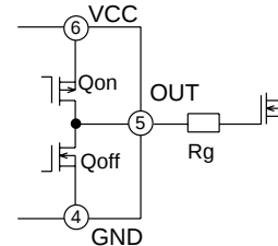
Fig. 35 Output Circuit (1)
