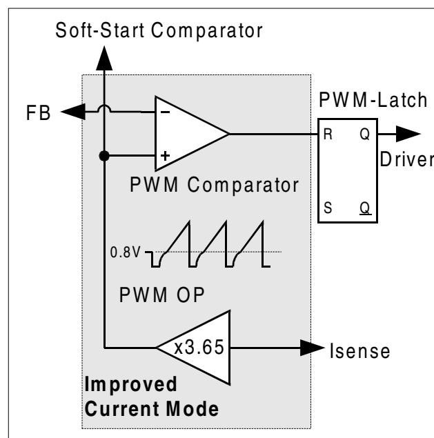
Current Mode means that the duty cycle is controlled by the slope of the primary current. This is done by comparison the FB signal with the amplified current sense signal.
